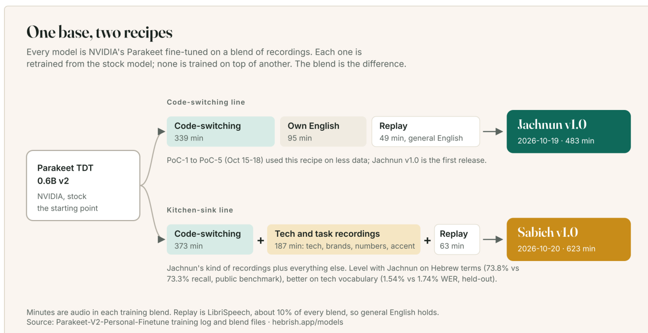
Figure 1. One base, two recipes. Minutes are audio in each training blend.
