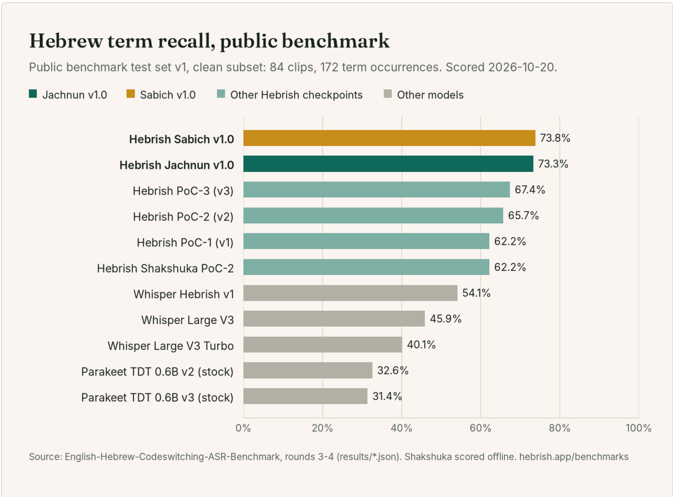
Figure 2. Hebrew term recall on the public benchmark, clean subset, all eleven scored models.
