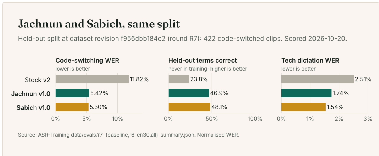
Figure 5. Stock v2, Jachnun v1.0 and Sabich v1.0 on the R7 held-out split. New in this edition.
