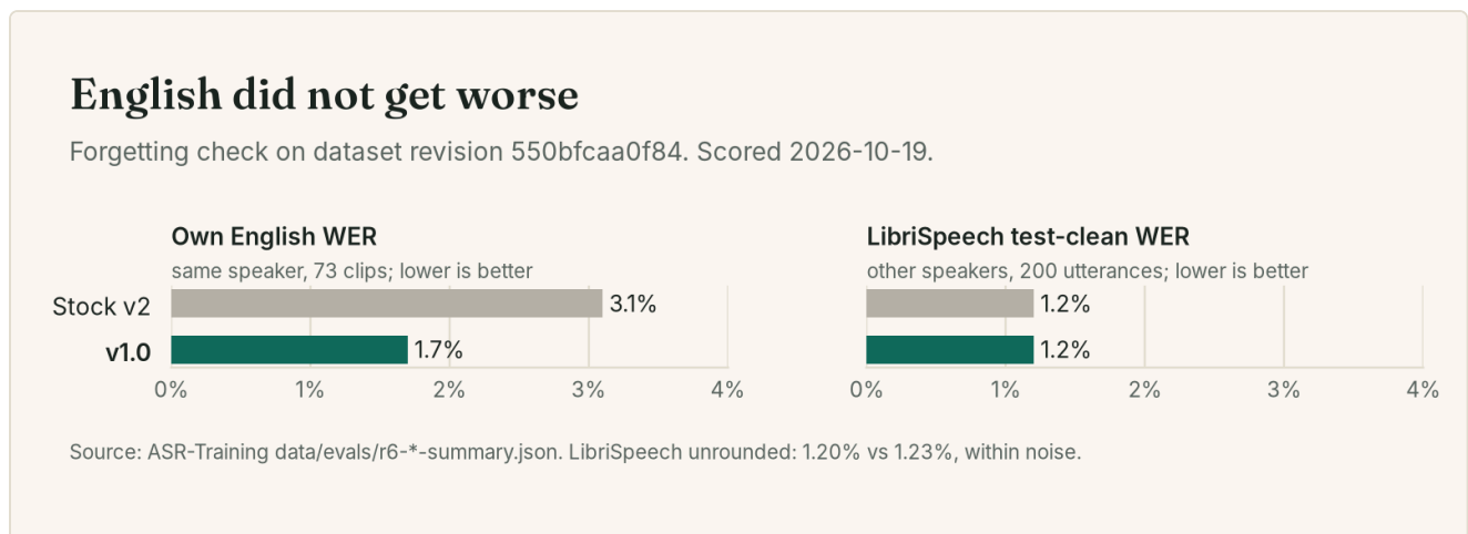
Figure 6. Forgetting check for Jachnun. Own English is the same speaker; LibriSpeech is other speakers.
