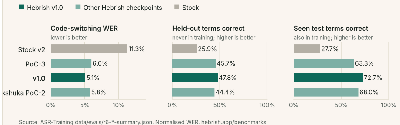
Figure 4. Stock v2, PoC-3, Jachnun v1.0 and Shakshuka PoC-2 on the same held-out split.
